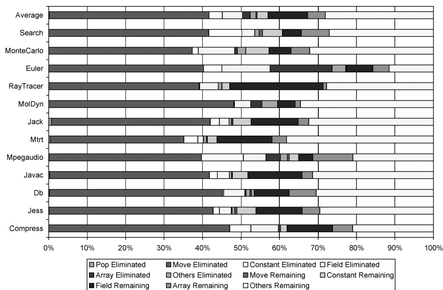
Fig. 21. Breakdown of dynamically appearing VM instructions with additional redundant heap load elimination for all the benchmarks. These results are indicative only, because our translator makes unsafe assumptions about aliasing.
