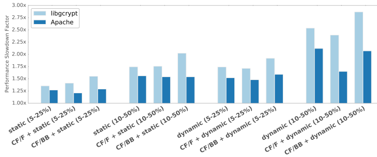
Figure 8: Performance slowdown factor. libgcrpt : AES micro-benchmark encryption performance slowdown, relative to a non-diversified baseline. Apache: slowdown when serving a 4MB file over HTTPS with AES block cipher, relative to a non-diversified baseline.
